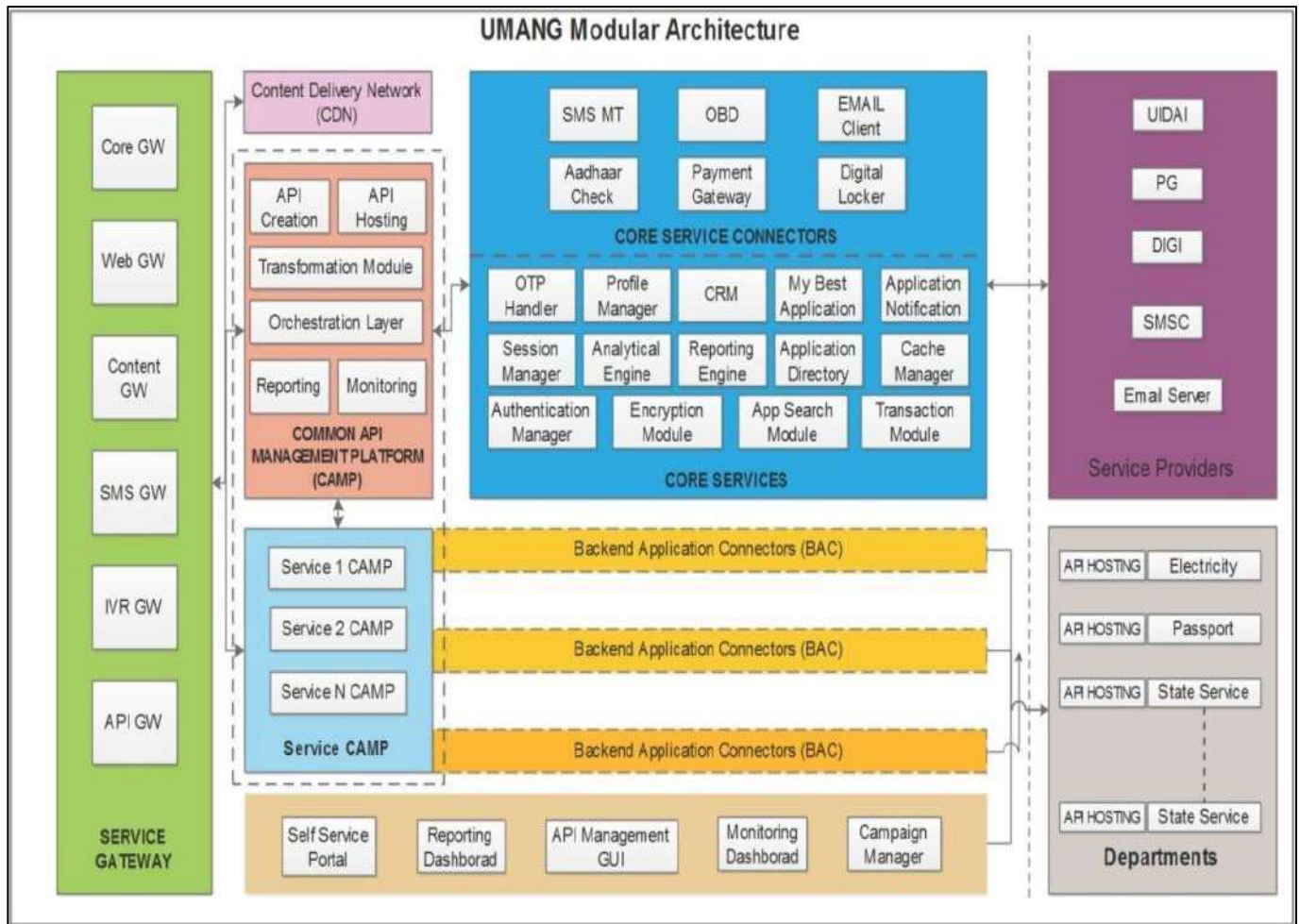
Fig 7 – UMANG Platform Architecture
